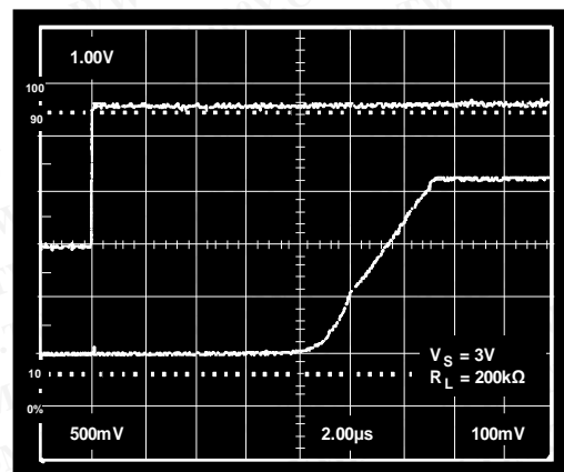
Figure 59. Large Signal Transient Response, V_S = 3V
