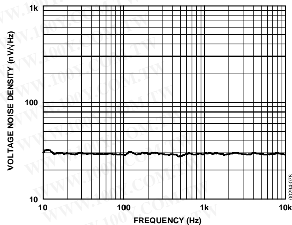
Figure 58. Voltage Noise Density, V_S = 3V
