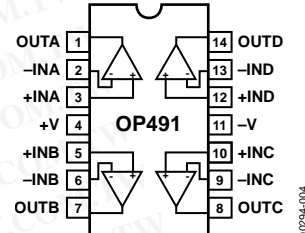
Figure 4. 14-Lead PDIP
