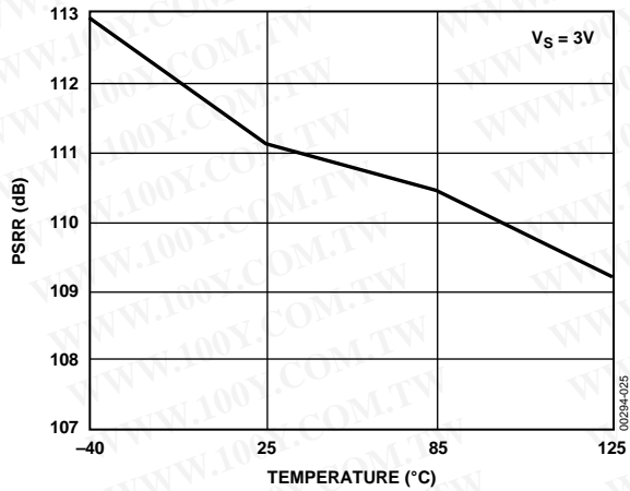
Figure 20. PSRR vs. Temperature, V_S = 3V
