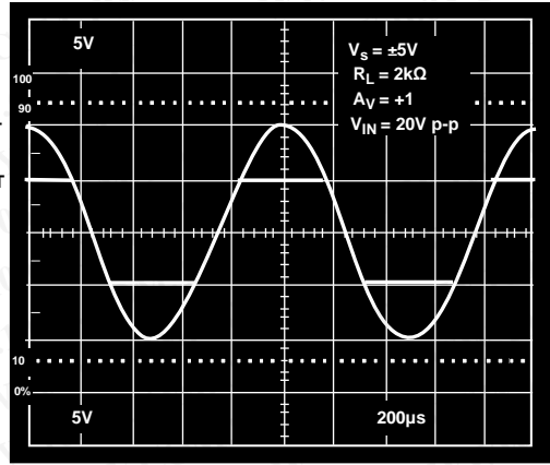
Figure 6. Input and Output with Inputs Overdriven by 5 V
