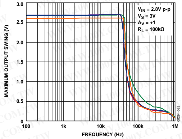
Figure 23. Maximum Output Swing vs. Frequency, V_S = 3V
