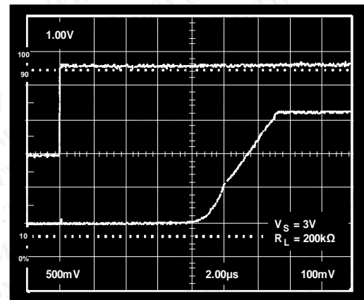
Figure 59. Large Signal Transient Response, V_S = 3V
