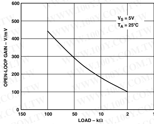
TPC 19. Open-Loop Gain vs. Resistive Load
