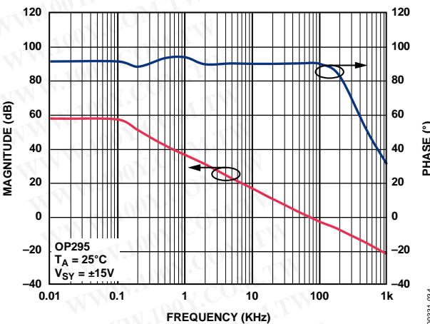
Figure 18. OP295 Gain and Phase vs. Frequency
