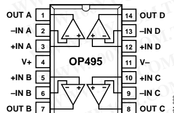
Figure 3. 14-Lead PDIP P Suffix (N-14)
