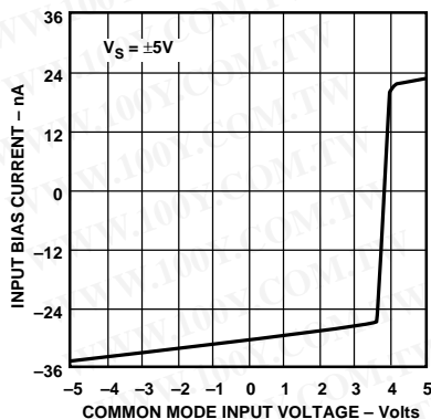
Figure 42. Input Bias Current vs. Common-Mode Voltage, V_S = \pm 5V
