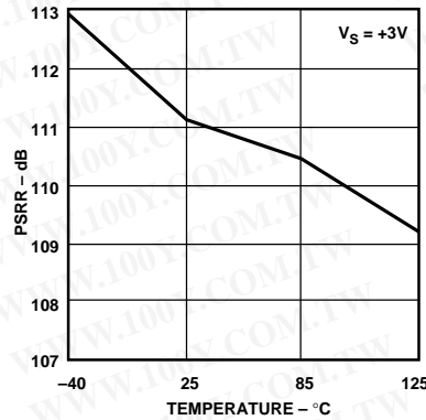
Figure 15. PSRR vs. Temperature, V_S = +3\text{ V}
