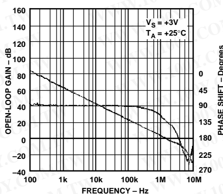
Figure 9. Open-Loop Gain & Phase vs. Frequency, V_S = +3V
