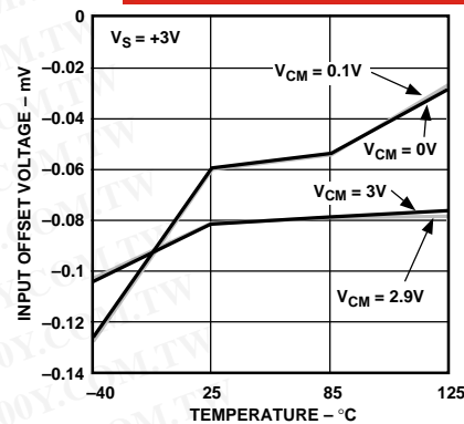
Figure 4. Input Offset Voltage vs. Temperature, V_S = +3V
