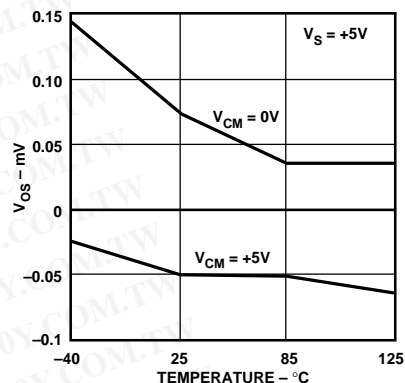
Figure 22. Input Offset Voltage vs. Temperature, V_S = +5\text{ V}
