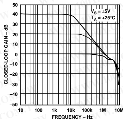
Figure 46. Closed-Loop Gain vs. Frequency, V_S = \pm 5V
