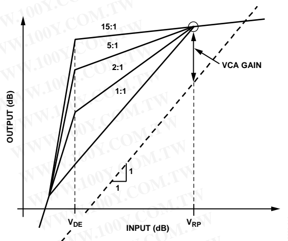
Figure 18. Effect of Varying the Compression Ratio
