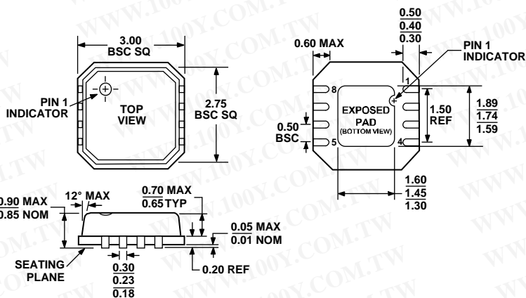
Figure 53. 8-Lead Lead Frame Chip Scale Package [LFCSP_VD] 3 mm × 3 mm Body, Very Thin, Dual Lead (CP-8-2)
