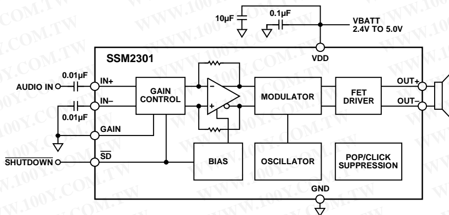
Figure 25. Single-Ended Input Configuration, Gain = 6 dB
