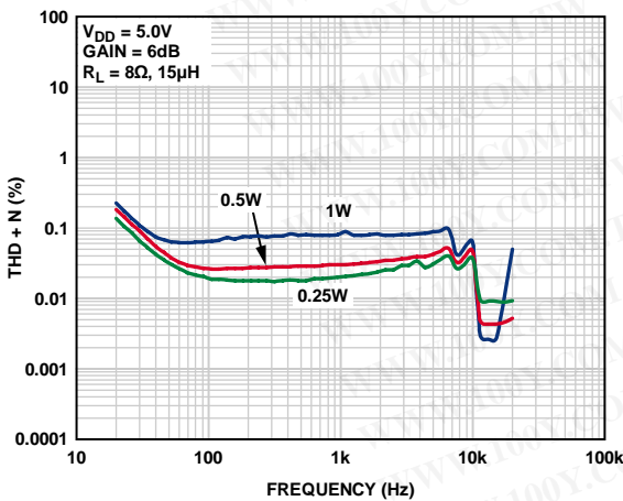
Figure 6. THD + N vs. Frequency, V_{DD} = 5.0V , A_V = 6dB , R_L = 8\Omega
