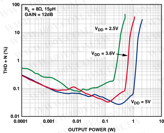
Figure 5. THD + N vs. Output Power into 8\Omega , A_V = 12dB
