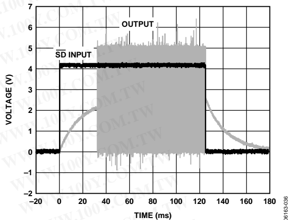
Figure 23. Turn-Off Response
