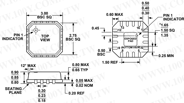
*COMPLIANT TO JEDEC STANDARDS MO-220-VEED-2 EXCEPT FOR EXPOSED PAD DIMENSION. Figure 47. 16-Lead Lead Frame Chip Scale Package [LFCSP_VQ] 3 mm × 3 mm Body, Very Thin Quad (CP-16-3) Dimensions shown in millimeters
