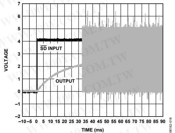
Figure 35. Turn-On Response
