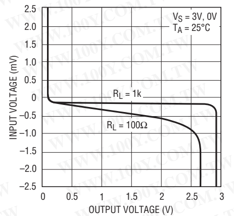
Open-Loop Gain
