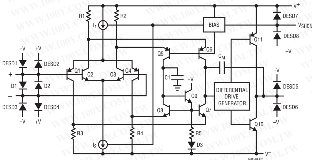
Figure 1. Simplified Schematic
