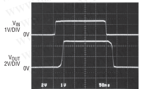
Output-Overdrive Recovery
