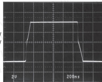
\pm 5V Large-Signal Response
