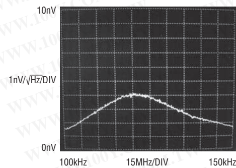
Input Referred High Frequency Noise Spectrum
