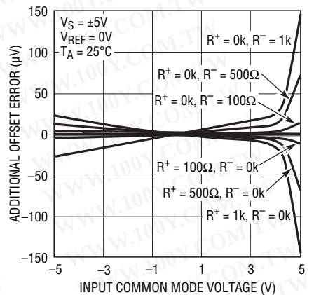
Error Due to Input R_S Mismatch vs Input Common Mode ( C_{IN} > 1\mu F )
