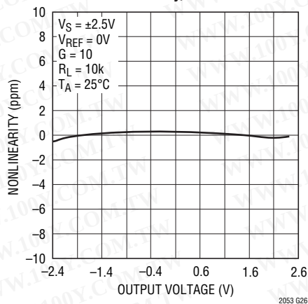
Gain Nonlinearity, G = 10
