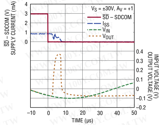
Shutdown Transient with Sinusoid Input
