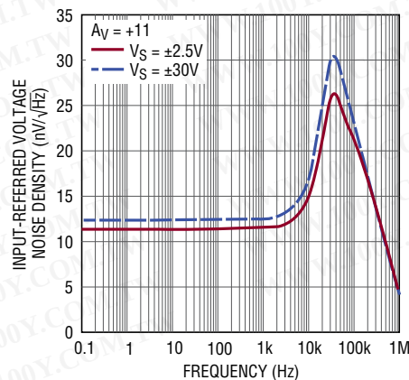
Input Voltage Noise Spectrum
