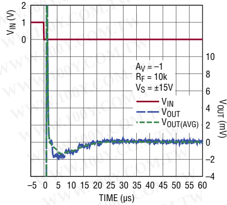
Large Signal Settling Transient
