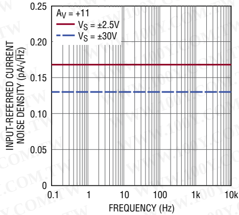
Input Current Noise Spectrum
