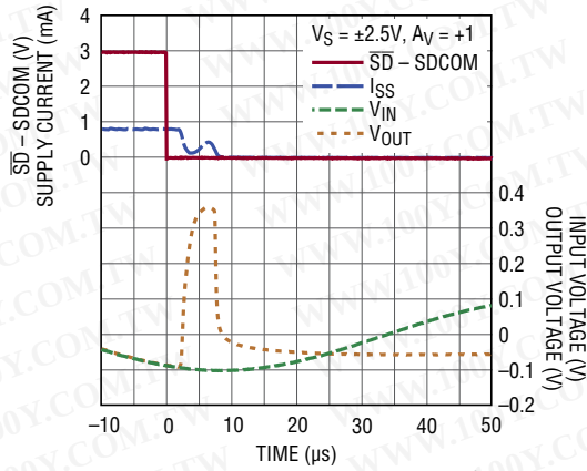
Shutdown Transient with Sinusoid Input
