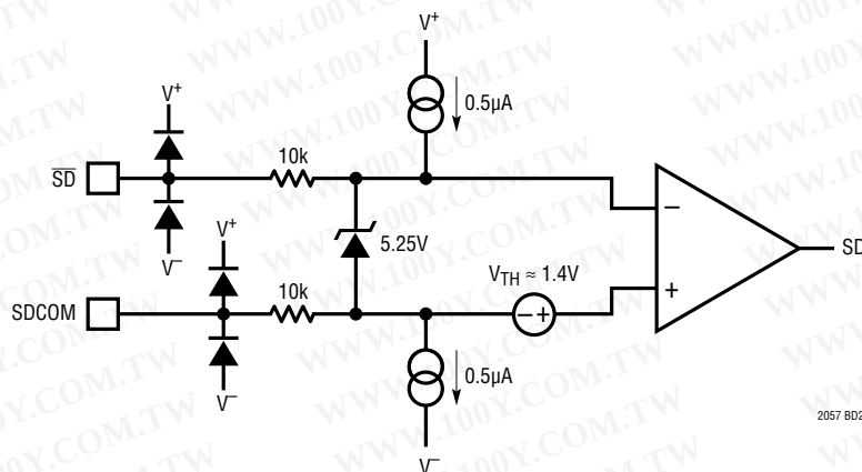
Shutdown Circuit
