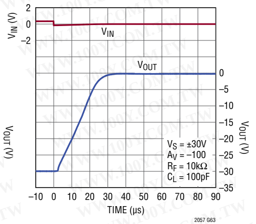
Output Overload Recovery
