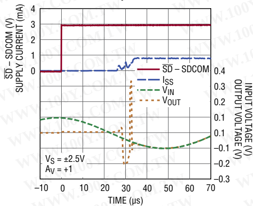
Start-Up Transient with Sinusoid Input
