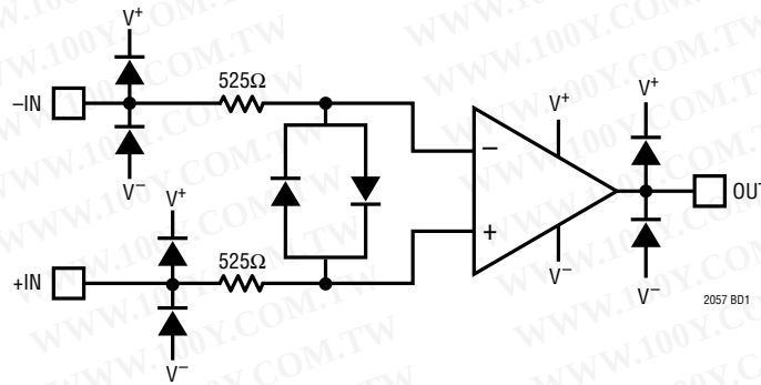
Amplifier
