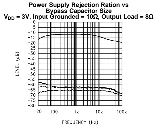
Figure 37. Top Trace = No Cap, Next Trace Down = 1µf Next Trace Down = 2µf, Bottom Trace = 4.7µf
