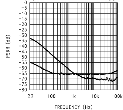
Figure 39. LM4890 = Bottom Trace LM4877 = Top Trace
