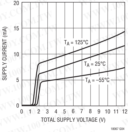
Supply Current per Amp vs Supply Voltage
