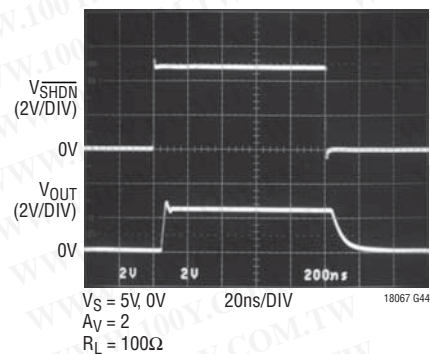
Shutdown Response
