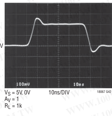
5V Small-Signal Response
