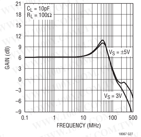
Gain vs Frequency (AV = 2)
