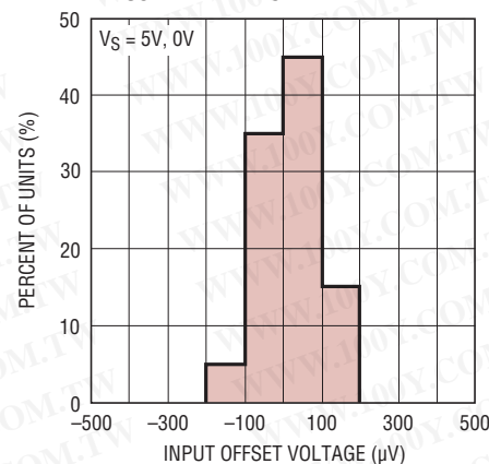
\Delta V_{\text{OS}} Shift for V_{\text{CM}} = 0\text{V} to 5\text{V}
