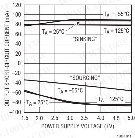
Output Short-Circuit Current vs Power Supply Voltage
