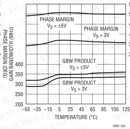
Gain Bandwidth and Phase Margin vs Temperature
