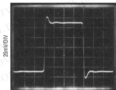
Small-Signal Transient Response VS = ± 2.5V
