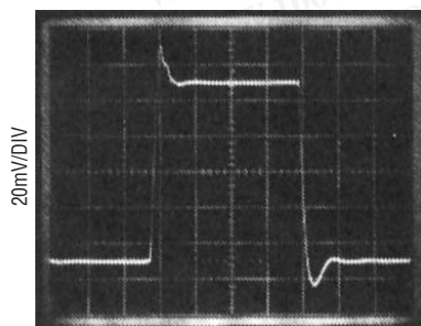
Small-Signal Transient Response VS = 5V, 0V
