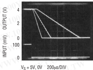
Comparator Fall Response Time to 10mV, 5mV, 2mV Overdrive
