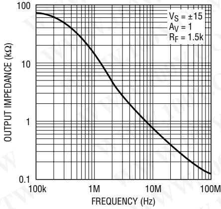
LT1259/60 • TPC11
