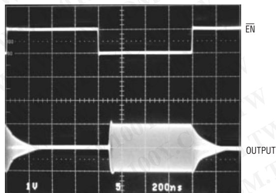
Amplifier Enable/Disable Time, A_V = 2
