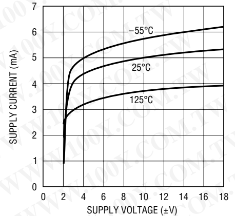
LT1259/60 • TPC13
