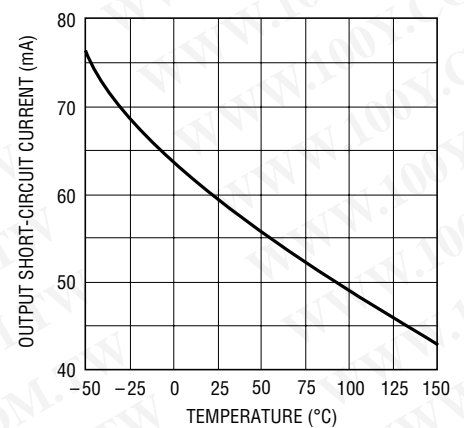
LT1259/60 • TPC15
