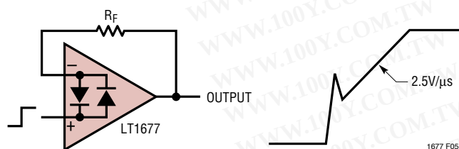
Figure 5. Pulsed Operation
