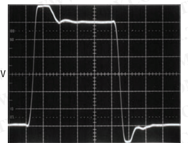
Large-Signal Transient, A_V = -1
