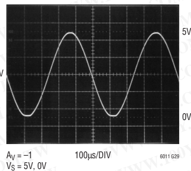
Rail-to-Rail Output Swing
