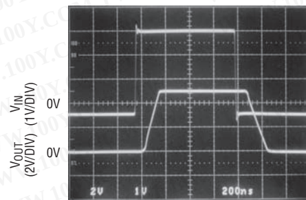
Output-Overdrive Recovery
