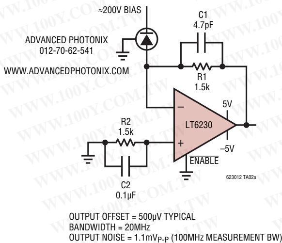
Low Power Avalanche Photodiode Transimpedance Amplifier I_S = 3.3\text{mA}
