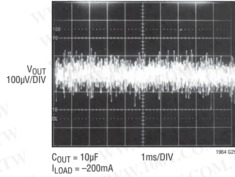
LT1964-5, 10Hz to 100kHz Output Noise, C_{BYP} = 0.01µF
