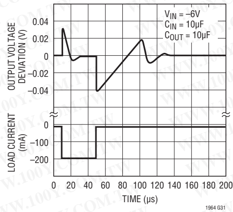
LT1964-5, Transient Response, C_{BYP} = 0.01µF
