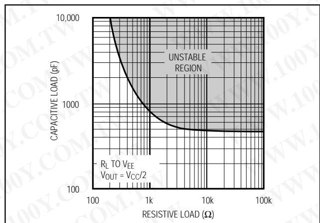
Figure 4. Capacitive-Load Stability
