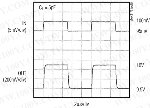
MAX4173H SMALL-SIGNAL TRANSIENT RESPONSE ( V_{SENSE} = 95mV to 100mV )
