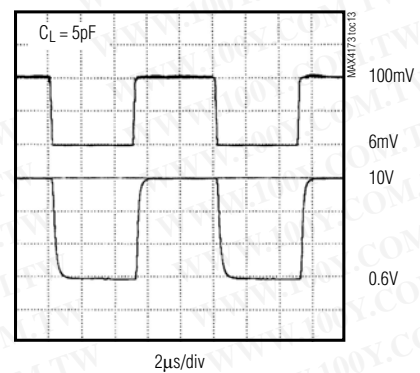
MAX4173H LARGE-SIGNAL TRANSIENT RESPONSE ( V_{SENSE} = 6mV to 100mV )
