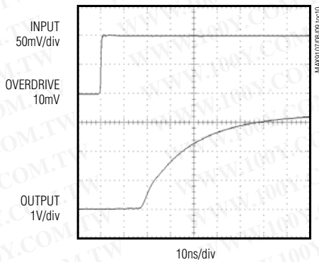
PROPAGATION DELAY ( t_{PD+} )
