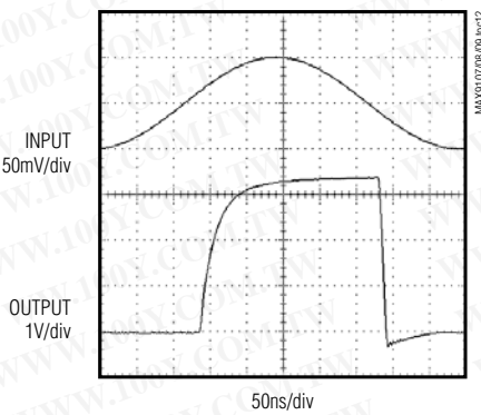
SINUSOID 2MHz RESPONSE
