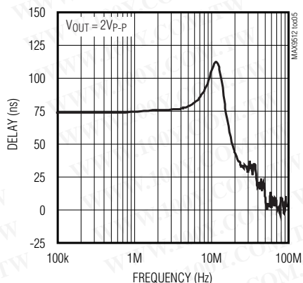
GROUP DELAY
