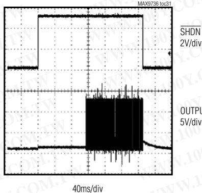
SHDN ON/OFF-RESPONSE
