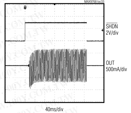
TURN-ON/OFF RESPONSE (MAX9768B)
