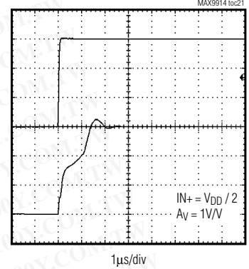
POWER-UP SETTLING TIME
