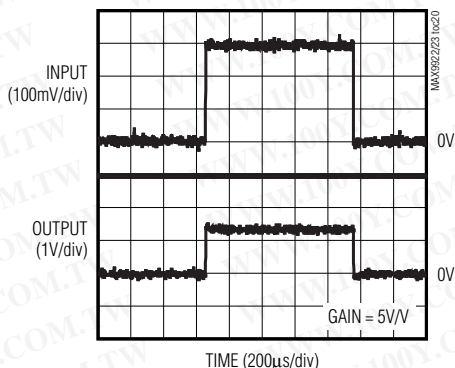
SATURATION/OVERLOAD RECOVERY (INPUT LIMITED) (MAX9922)
