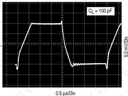
Figure 25. Large Signal
