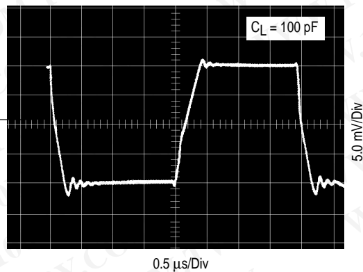
Figure 27. Large Signal
