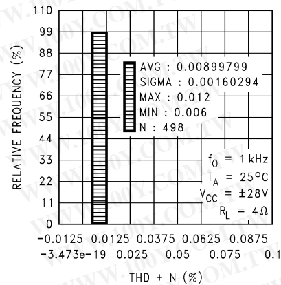
THD + N Distribution
