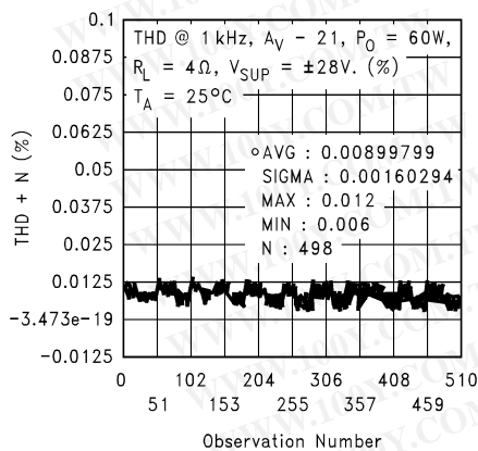
THD + N Distribution
