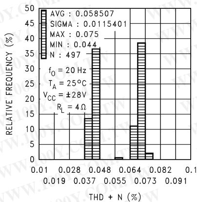
THD + N Distribution
