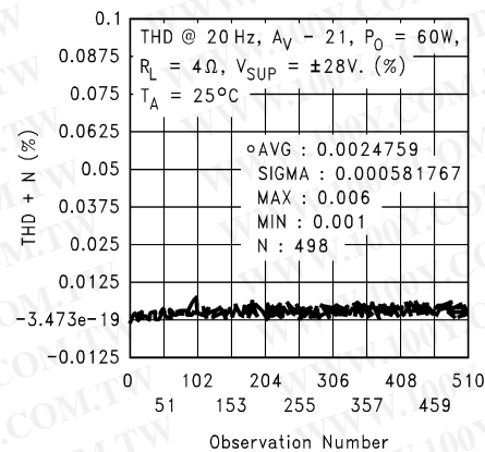
THD + N Distribution
