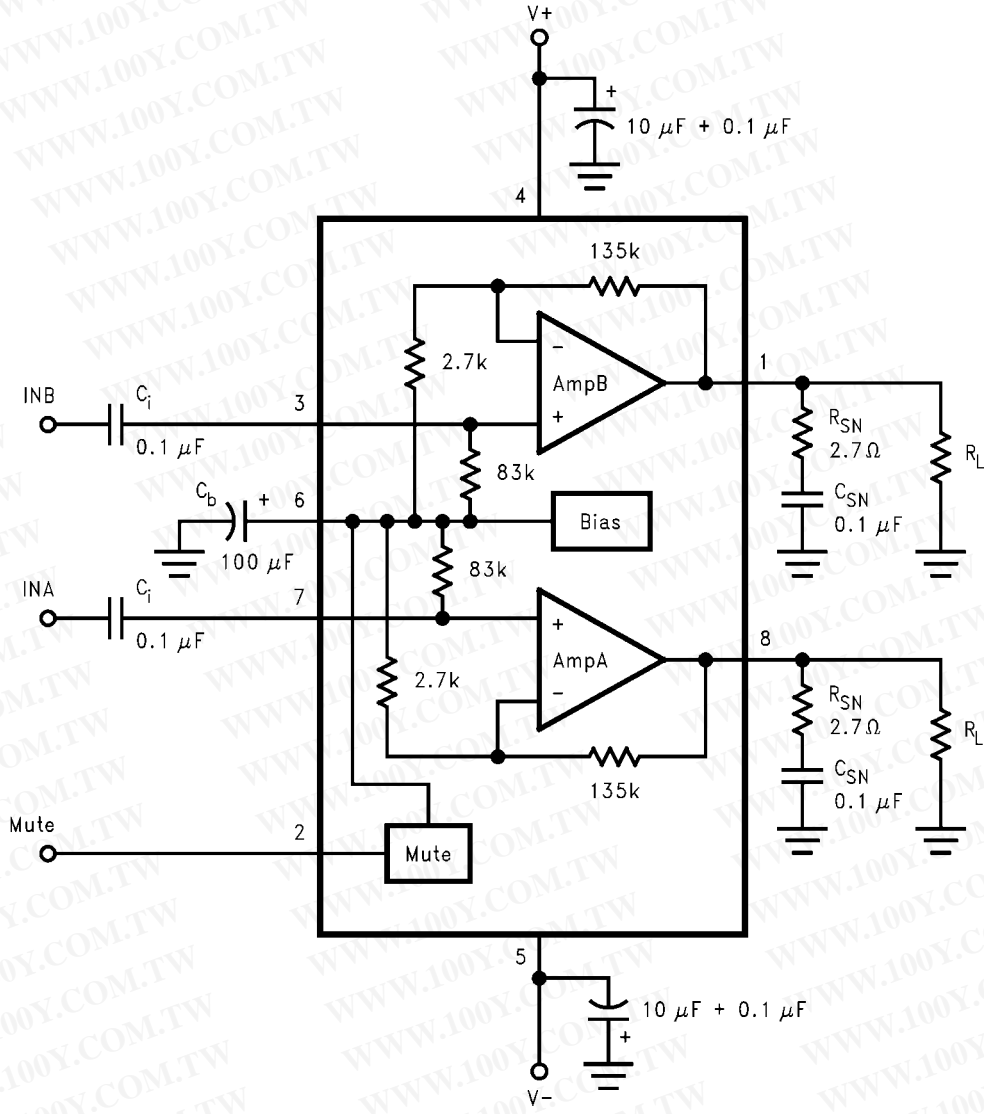
FIGURE 2. Test Circuit
