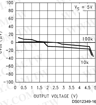
dV_{OS} vs Output Voltage
