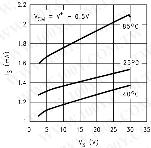
I_S vs. V_S (NPN side)
