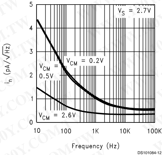
Input Noise Current for Various V_{CM}
