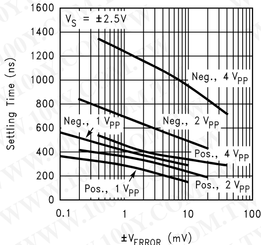
Settling Time vs. Error Voltage
