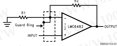
Non-Inverting Amplifier
