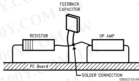
FIGURE 11. Air Wiring
