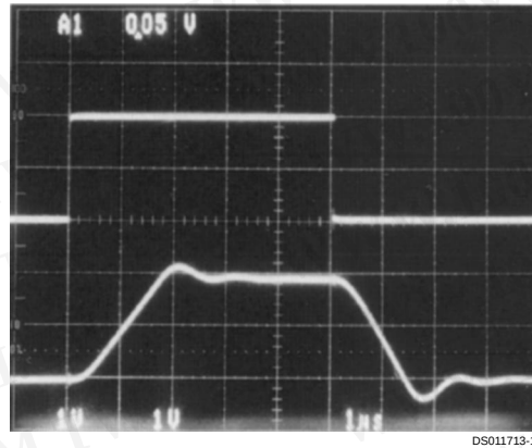
FIGURE 7. Pulse Response of LMC6482 Circuit in Figure 6
