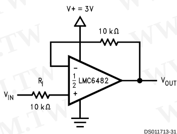
FIGURE 17. Half-Wave Rectifier with Input Current Protection (RI)
