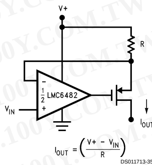
FIGURE 21. Large Compliance Range Current Source
