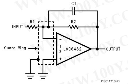
Inverting Amplifier
