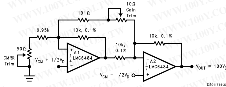
FIGURE 16. Low-Power Two-Op-Amp Instrumentation Amplifier
