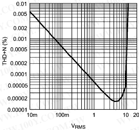
THD+N vs Output Voltage V_{CC} = 17V, V_{EE} = -17V, R_L = 2k\Omega
