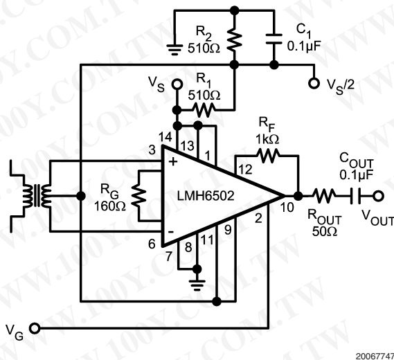
FIGURE 5. Transformer Coupled Single Supply VGA
