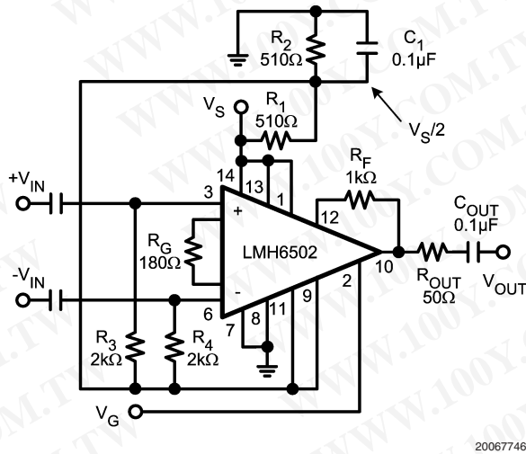
FIGURE 4. AC Coupled Single Supply VGA
