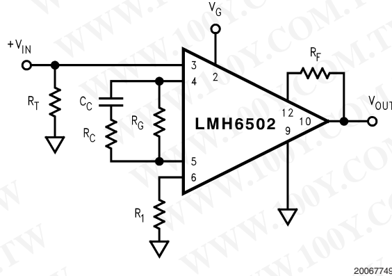
FIGURE 7. Frequency Shaping
