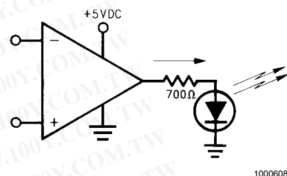
FIGURE 23. LED Driver
