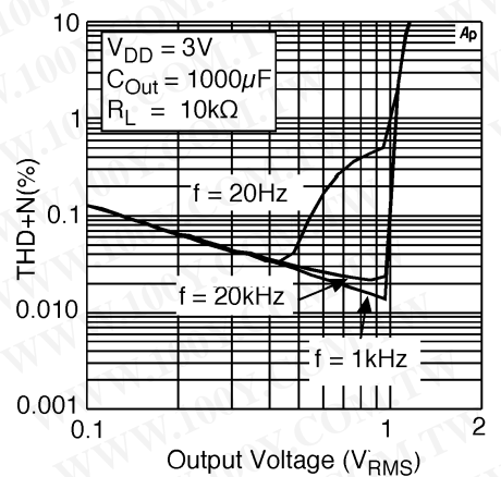
THD+N vs Output Voltage Docking Station Pins
