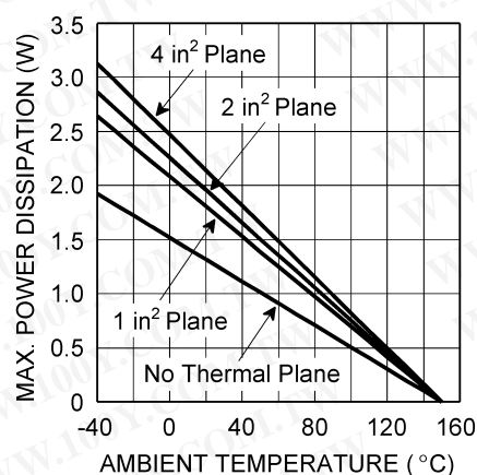
LM4838ITL (Note 19) Power Derating Curve
