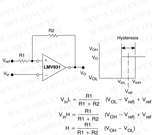
Figure 31. Comparator with Hysteresis
