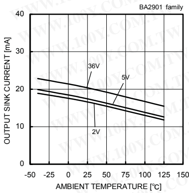
Fig.7 Output Sink Current - Ambient Temperature (VOL=1.5[V])
