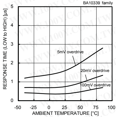
Fig. 19 Response Time LH – Ambient Temperature (VCC=5[V], VRL=5[V], RL=5.1[kΩ])
