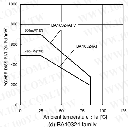
Fig. 125 Thermal resistance and derating
