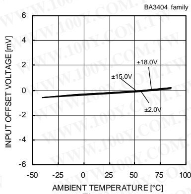
Fig. 104 Input Offset Voltage - Ambient Temperature (V icm =0[V], V OUT =0[V])
