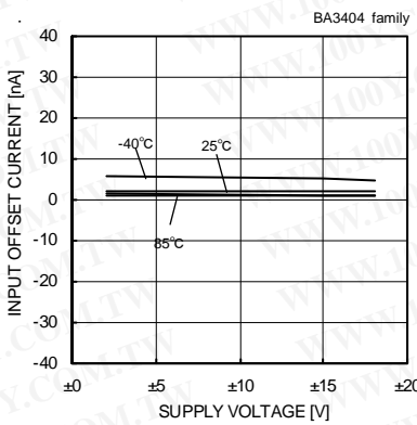
Fig. 107 Input Offset Current - Supply Voltage (V icm =0[V], V OUT =0[V])
