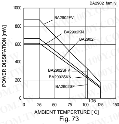
Derating Curve
