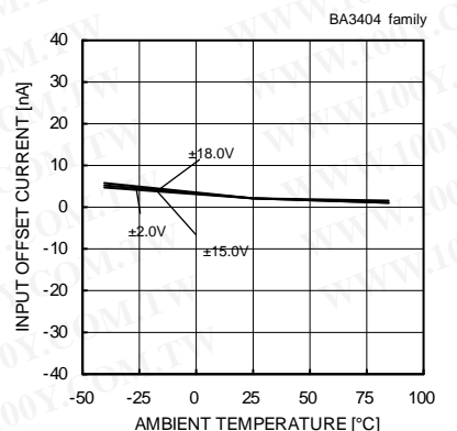
Fig. 108 Input Offset Current - Ambient Temperature (V icm =0[V], V OUT =0[V])
