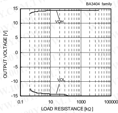
Fig. 100 Maximum Output Voltage - Load Resistance (V CC /V EE =+15[V]/-15[V], T a =25[°C])
