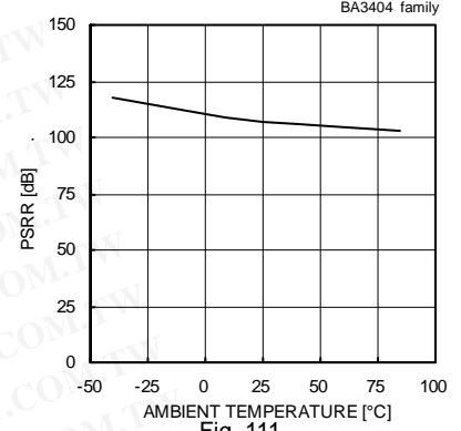
Power Supply Rejection Ratio - Ambient Temperature (VCC/VEE=+15[V]/-15[V])
