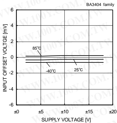
Fig. 103 Input Offset Voltage - Supply Voltage (V icm =0[V], V OUT =0[V])
