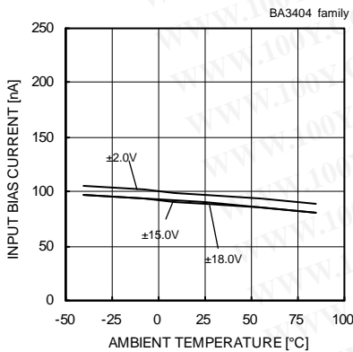
Fig. 106 Input Bias Current - Ambient Temperature (V icm =0[V], V OUT =0[V])
