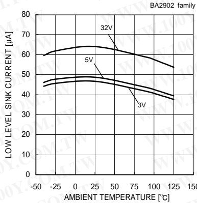
Low Level Sink Current - Ambient Temperature (VOUT=0.2[V])
