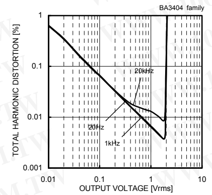
Total Harmonic Distortion - Output Voltage (VCC/VEE=+4[V]/-4[V], Av=0[dB], RL=2[kΩ], 80[kHz]-LPF, Ta=25°C)
