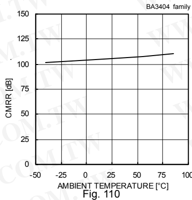
Common Mode Rejection Ratio - Ambient Temperature (VCC/VEE=+15[V]/-15[V])
