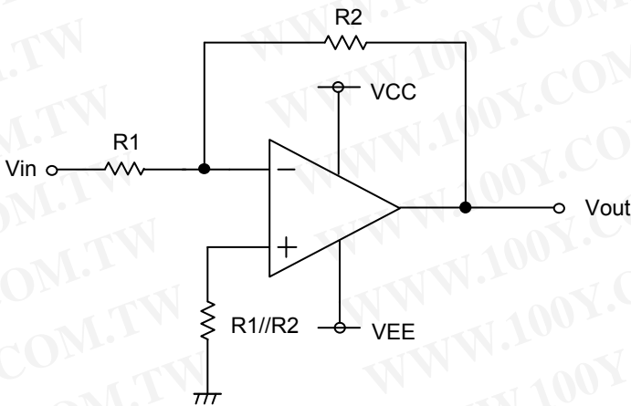
○ Inverting amplifier
