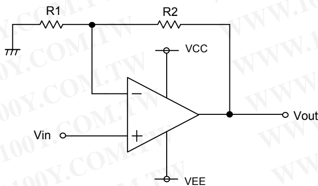
○ Non-inverting amplifier
