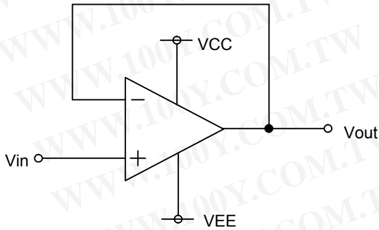
○ Voltage follower
