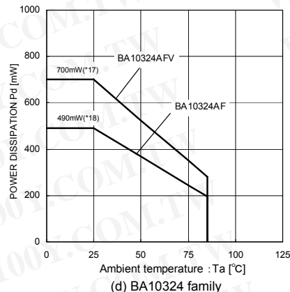
Fig. 125 Thermal resistance and derating
