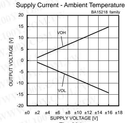
Maximum Output Voltage - Supply Voltage (RL=2[kΩ], Ta=25[°C])
