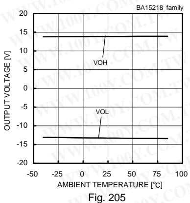
Maximum Output Voltage - Ambient Temperature (VCC/VEE=+15[V]/-15[V], RL=2[kΩ])
