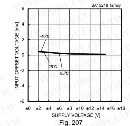
Input Offset Voltage - Supply Voltage (Vicm=0[V], Vout=0[V])
