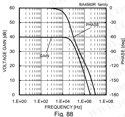
Fig. 88 Voltage Gain - Frequency ( V_{CC}/V_{EE}=+15[V]/-15[V] , A_v=40[dB] , R_L=2[k\Omega] , T_a=25[^\circ C] )
