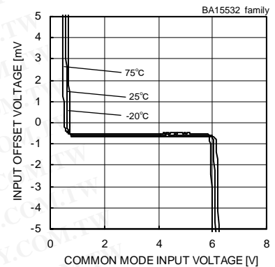
Fig. 257 Input Offset Voltage - Common Mode Input Voltage ( V_{CC}=8[V] , V_{out}=4[V] )
