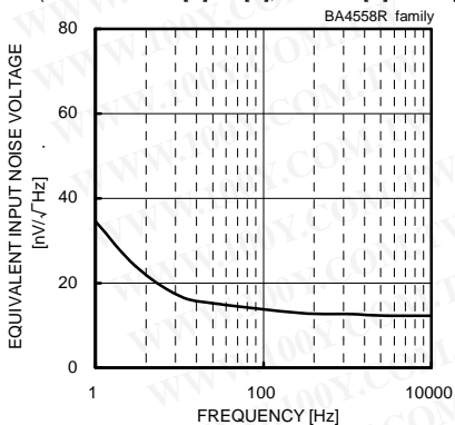
Equivalent Input Noise Voltage - Frequency ( V_{CC}/V_{EE}=+15[V]/-15[V] , R_s=100[\Omega] , T_a=25[^\circ C] )
