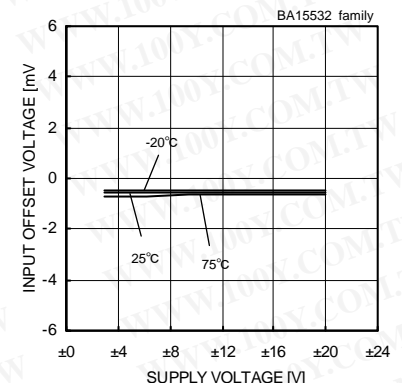
Fig. 251 Input Offset Voltage - Supply Voltage (Vicm=0[V], Vout=0[V])
