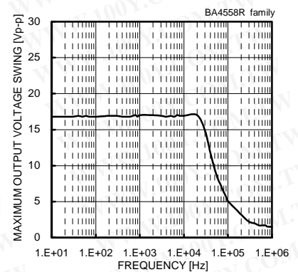
Maximum Output Voltage Swing - Frequency ( V_{CC}/V_{EE}=+15[V]/-15[V] , R_L=2[k\Omega] , T_a=25[^\circ C] )
