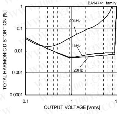
Fig. 240 Total Harmonic Distortion - Output Voltage ( V_{CC}/V_{EE}=+15[V]/-15[V] , A_v=20[dB] , R_L=2[k\Omega] , 80[kHz] -LPF, T_a=25[^\circ C] )
