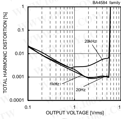
Fig. 152 Total Harmonic Distortion - Output Voltage ( V_{CC}/V_{EE}=+15[V]/-15[V] , A_v=20[dB] , R_L=2[k\Omega] , 80[kHz] -LPF, T_a=25[^\circ C] )
