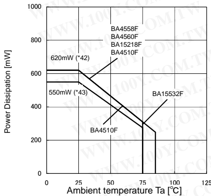
(e)BA4558/BA4560/BA15218/BA15532/BA4510 family
