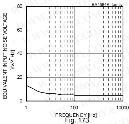
Equivalent Input Noise Voltage - Frequency (V CC /V EE =+9.5[V]/-9.5[V], R s =100[Ω], T a =25[°C])
