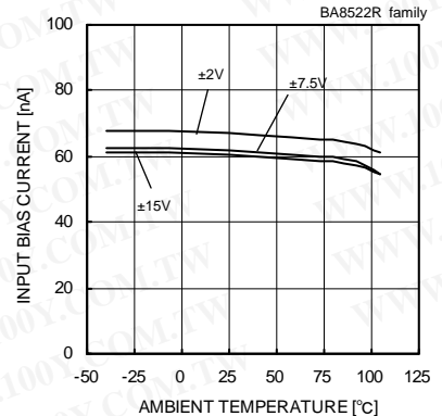
Fig. 188 Input Bias Current - Ambient Temperature (Vicm=0[V], Vout=0[V])
