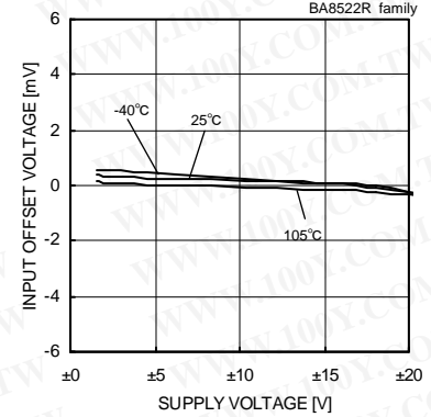
Fig. 185 Input Offset Voltage - Supply Voltage (Vicm=0[V], Vout=0[V])
