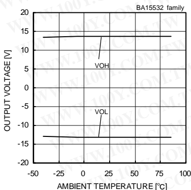
Fig. 249 Maximum Output Voltage - Ambient Temperature (VCC/VEE=+15[V]/-15[V], RL=2[kΩ])
