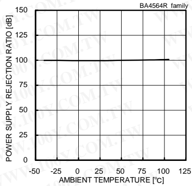
Fig. 105 Power Supply Rejection Ratio - Ambient Temperature ( V_{CC}/V_{EE}=+4[V]/-4[V] to +15[V]/-15[V] )
