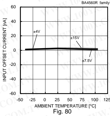
Fig. 80 Input Offset Current - Ambient Temperature ( V_{icm}=0[V] , V_{out}=0[V] )
