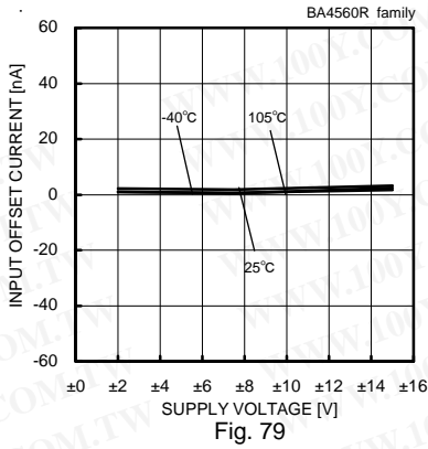
Fig. 79 Input Offset Current - Supply Voltage ( V_{icm}=0[V] , V_{out}=0[V] )
