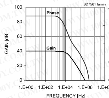
Fig. 23 Gain - Frequency
