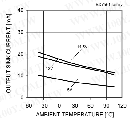
Fig. 12 Output Sink Current - Ambient Temperature (VOUT=VDD-11.6[V])
