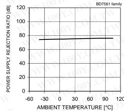
Fig. 20 Power Supply Rejection Ratio – Ambient Temperature
