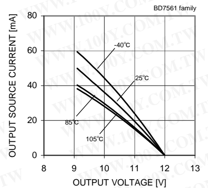
Fig. 9 Output Source Current - Output Voltage (VDD=12[V])
