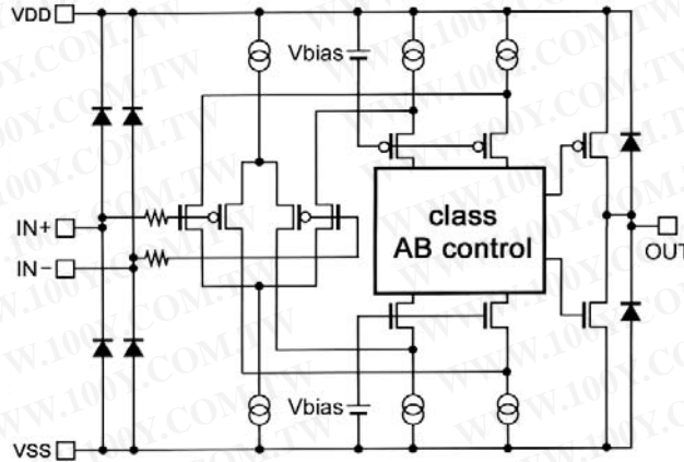
Fig. 93. Schematic diagram
