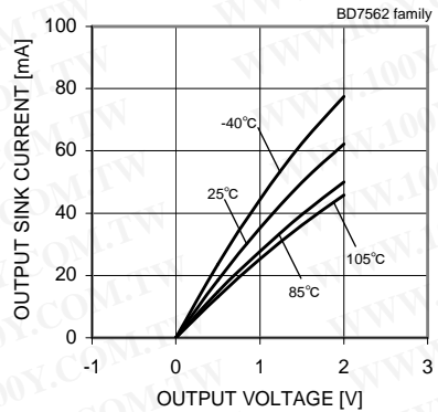
Fig. 34 Output Sink Current - Output Voltage (VDD=12[V])
