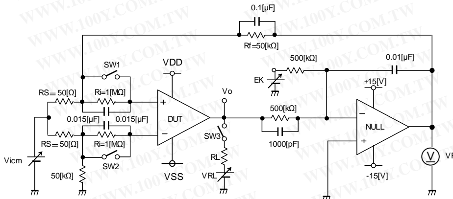
Fig. 94. Test circuit 1 (one channel only)
