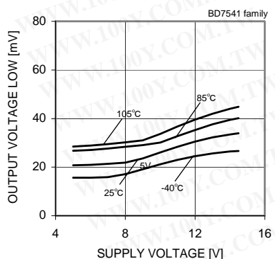
Fig. 53 Output Voltage Low – Supply Voltage ( R_L=10[k\Omega] )
