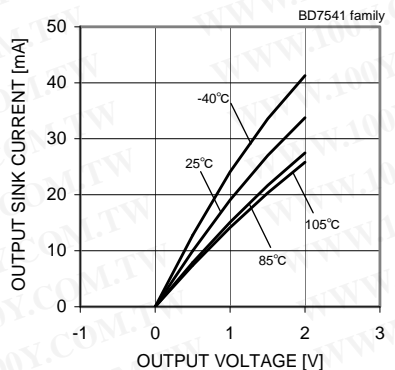
Fig. 57 Output Sink Current – Output Voltage ( V_{DD}=12[V] )
