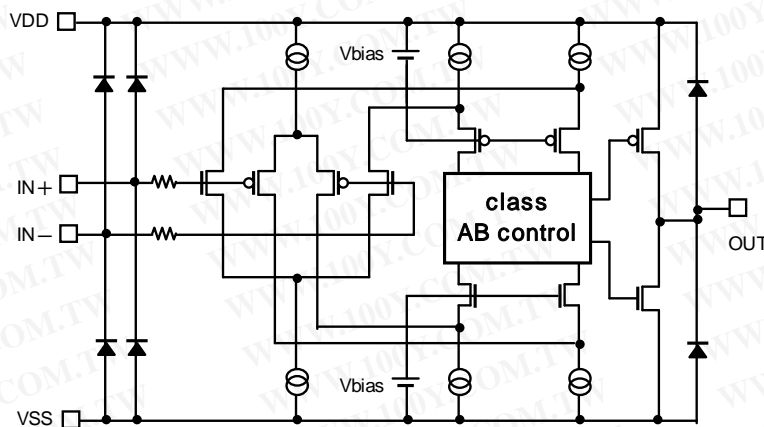
Fig.189 Simplified schematic
