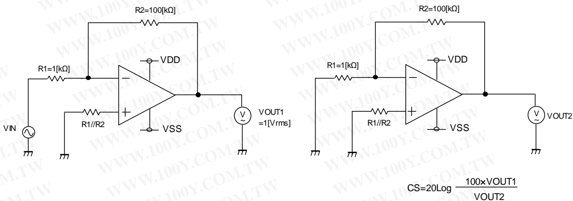
Fig.188 Test circuit 3
