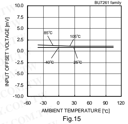
Fig.15 Input Offset Voltage – Ambient Temperature (VDD=3[V])
