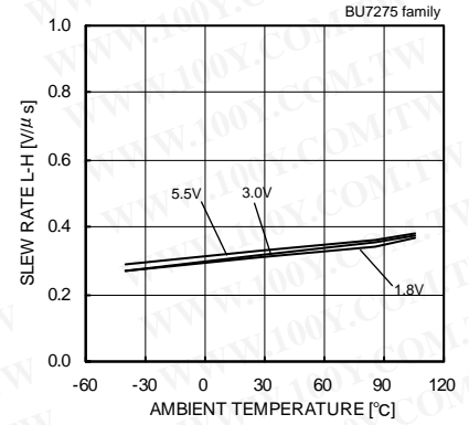
Fig.182 Slew Rate L-H – Ambient Temperature
