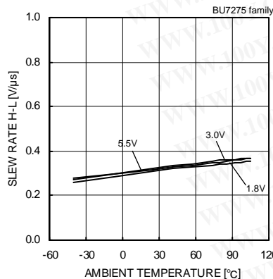
Fig.183 Slew Rate H-L – Ambient Temperature
