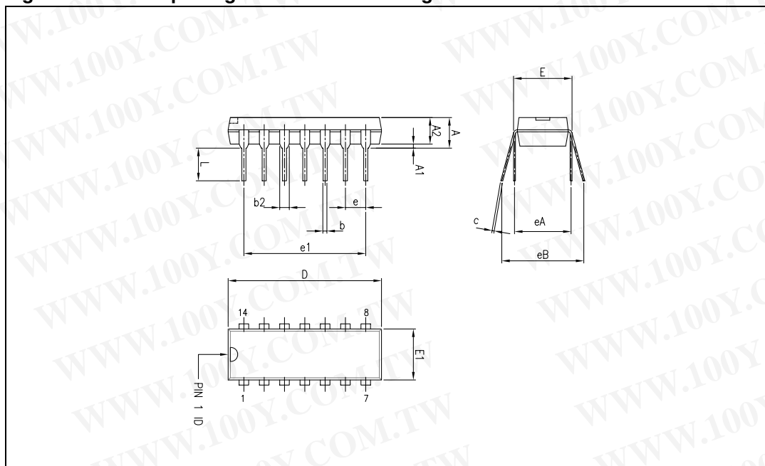
Figure 22. DIP14 package mechanical drawing
