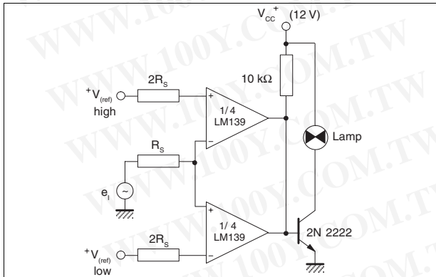
Figure 18. Limit comparator
